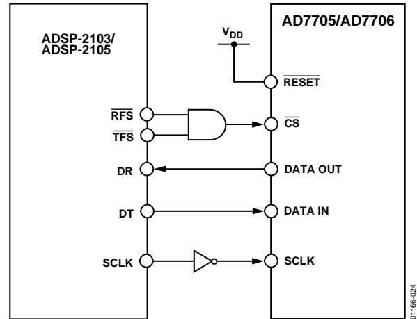
Figure 24. AD7705/AD7706-to-ADSP-2103/ADSP-2105 Interface
