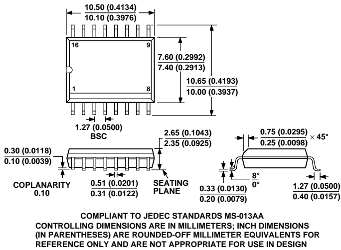
Figure 30. 16-Lead Standard Small Outline Package [SOIC] Wide Body (R-16) Dimensions shown in millimeters and (inches)
