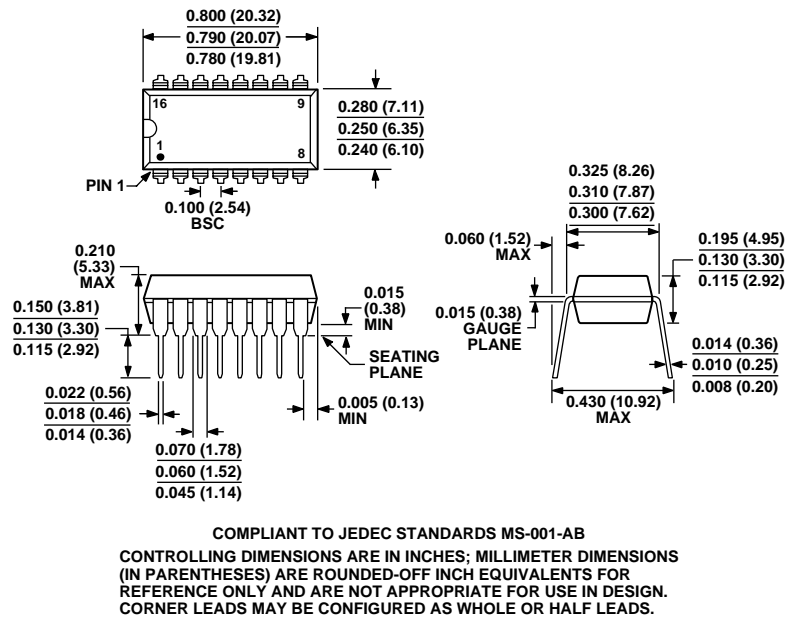
Figure 32. 16-Lead Plastic Dual In-Line Package [PDIP] Narrow Body (N-16) Dimensions shown in inches and (millimeters)
